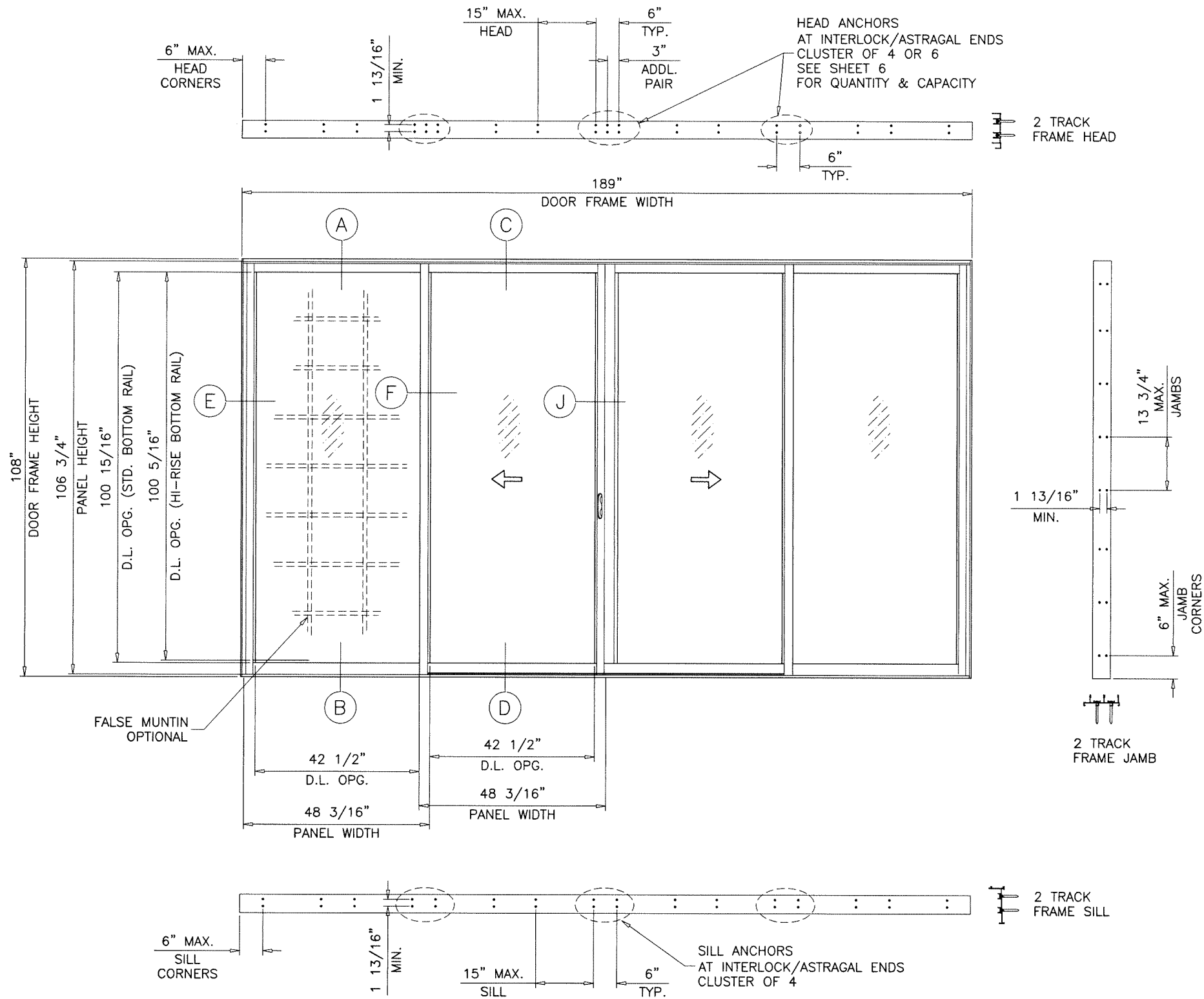
TYPICAL ELEVATION OX-XO
